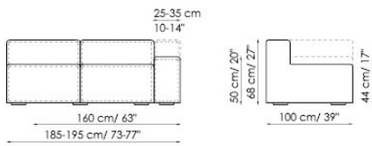
Terminale 185/195 End section Prof.100 depth dx right
