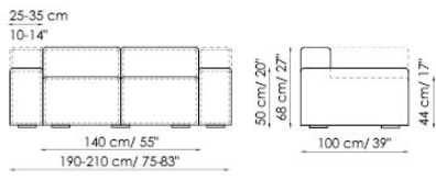
Divano 190/210 Sofa Prof.100 depth
