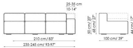
Terminale 235/245 End section Prof.100 depth dx right
